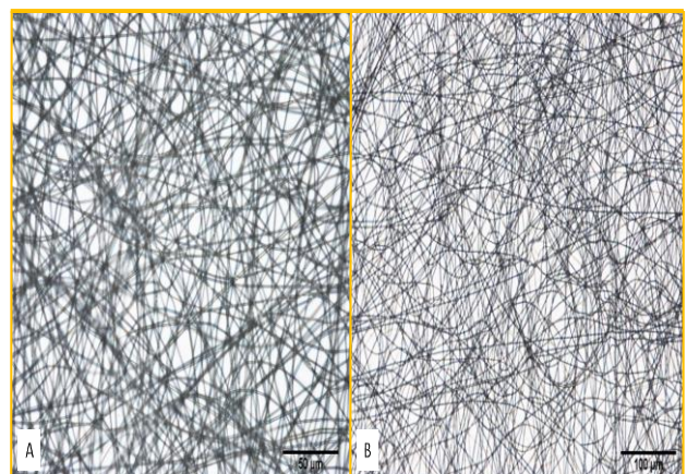
Figure 2 (A and B): Light microscopy of electrospun nanofibers. Optical microscopy of nanofibers with a 50 µm scale, 100 µm scale.
